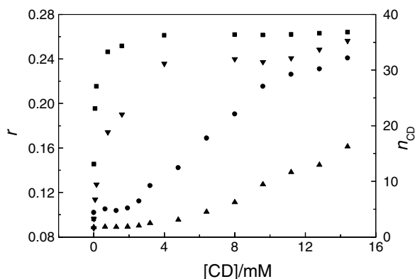
Fig. 3. Steady-state fluorescence anisotropy of BOS at the concentration of 1 \times 10^{-6} M (● \beta -CD, ■ \gamma -CD), and the average number of CD in the nanotube (▲ \beta -CD, ▼ \gamma -CD).
