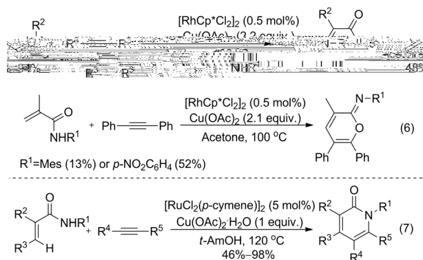
Scheme 29 Rh(III)-catalyzed oxidative coupling of acrylamides with alkynes.
