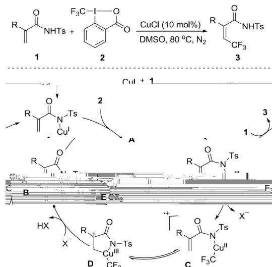
Scheme 20 Cu(I)-mediated trifluoromethylation of acrylamides.
