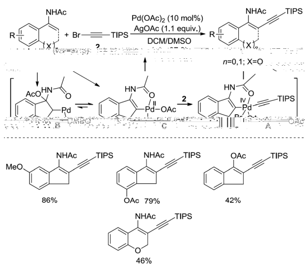
Scheme 7 Pd(II)-catalyzed directed alkynylation of N -vinylacetamides.
