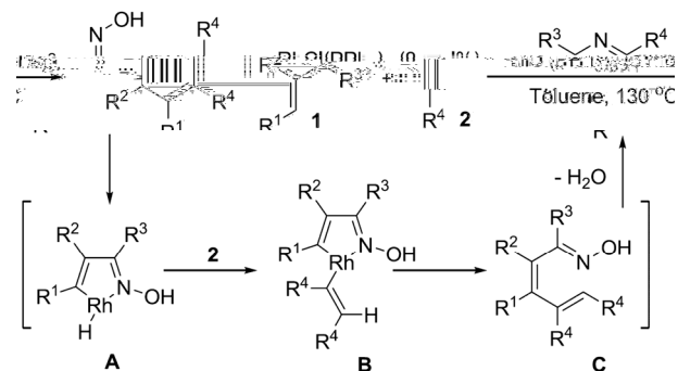
Scheme 27 Rh(I)-catalyzed synthesis of substituted pyridines from \alpha,\beta -unsaturated ketoximes and alkynes.
