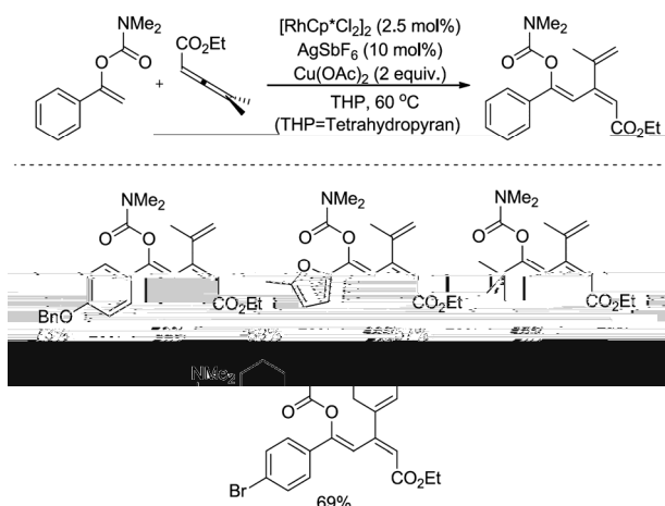
Scheme 14 Rh(III)-catalyzed C–H activation of enolate esters with alkenes to conjugated olefins.
