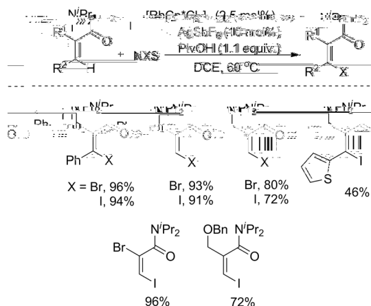
Scheme 25 Rh(III)-catalyzed halogenation of vinyl C-H bonds.
