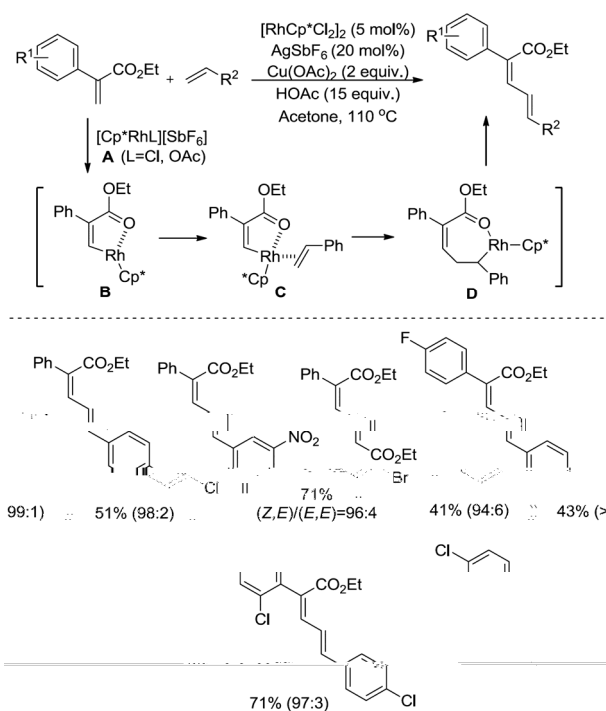
Scheme 11 Ester-directed selective olefination of acrylates by Rh(III) catalysis.
