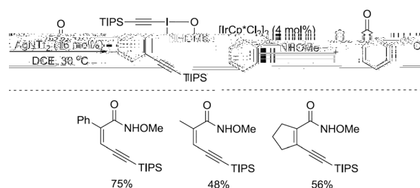
Scheme 4 Ir(III)-catalyzed alkynylation of acrylamide derivatives.
