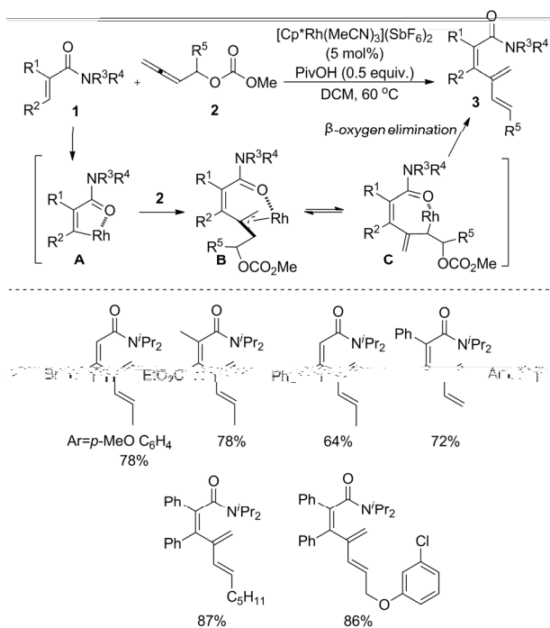
Scheme 13 Rh(III)-catalyzed C–H activation/functionalization of acrylamides with allenyl carbinol carbonates.
