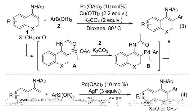
Scheme 15 Pd(II)-catalyzed arylation of cyclic enamides with arylboronic acids and arylsilanes.
