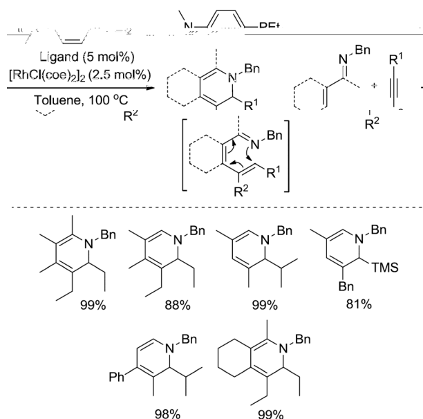
Scheme 26 Rh(III)-catalyzed synthesis of dihydropyridines from imines and alkynes.
