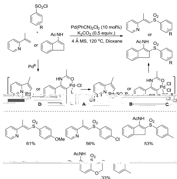
Scheme 24 Pd(II)-catalyzed sulfonylation of alkenyl C–H bonds using organosulfonyl chlorides.
