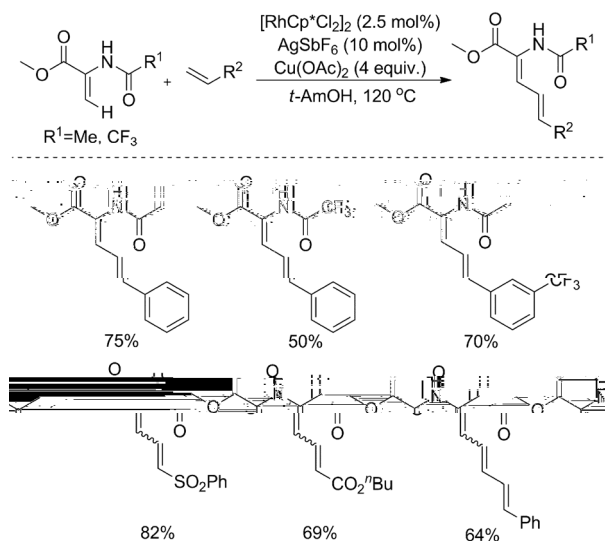
Scheme 9 Rh(III)-catalyzed olefination of acrylamides and acrylates with styrenes and acrylates.
