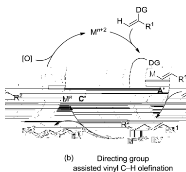
Scheme 8 Synthesis of dienes via oxidative Heck reaction (a) or directed vinylic C–H activation (b).
